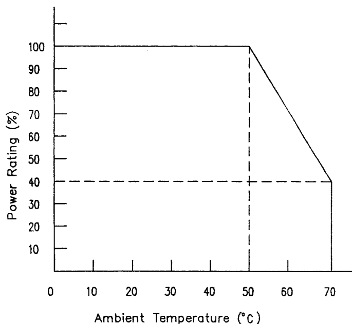
FIGURE 3 PERCENT POWER RATING VERSUS AMBIENT TEMPERATURE
