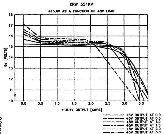
FIGURE 2 +15.6V OUTPUT AS A FUNCTION OF +5V LOAD
