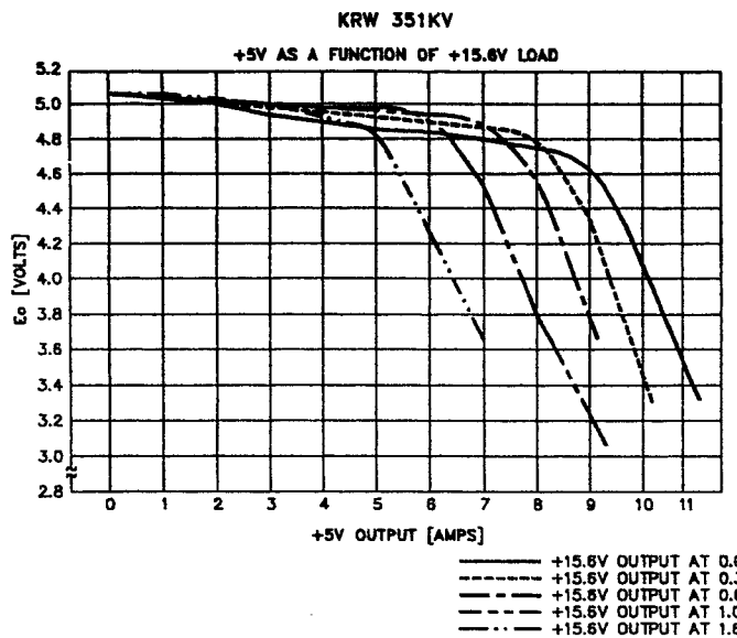
FIGURE 1 +5 V OUTPUT AS A FUNCTION OF +15.6V LOAD
